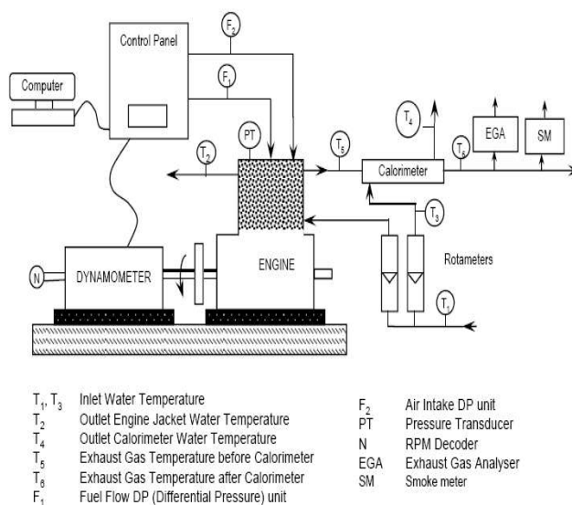
Figure 4: Experimental setup of Diesel engine
