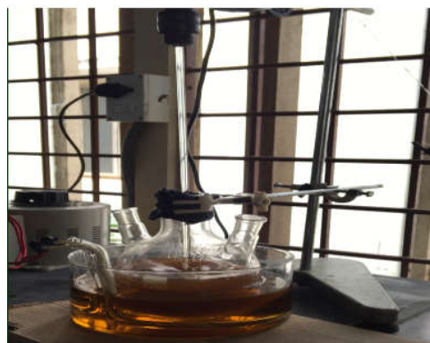
Figure 1: Transesterification
