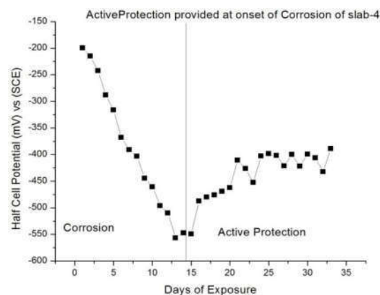
Fig. 5 Corrosion and Active Protection provided on block[10]
