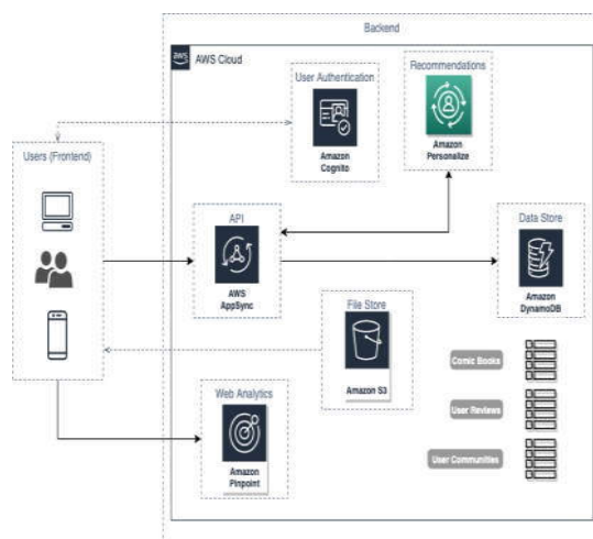
Fig.2 AWS FLOWCHART
